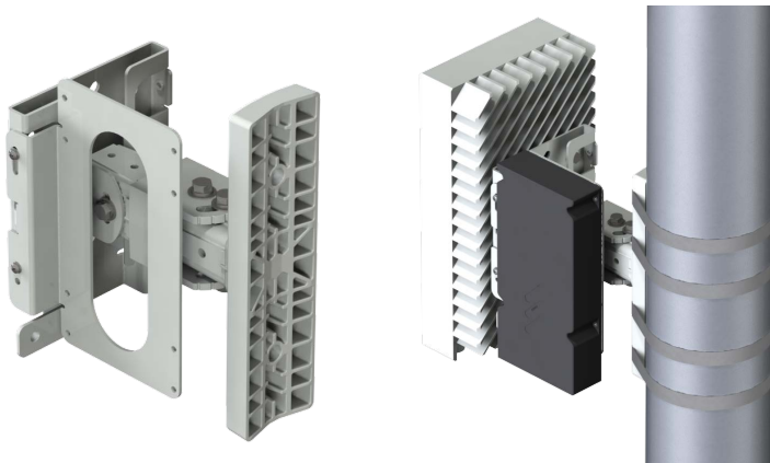
PTS5G-BK5201-V2E SINGLE RADIO MOUNT for 4435 5G radio and shown with included OAD Bracket
