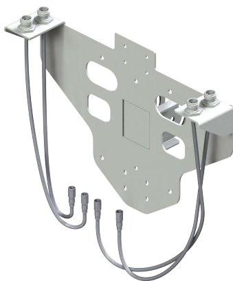
PTS5G-BK5112 OMNI Bracket for Ericsson 4G 2202 or 4402 only 2 Dual 2 GHz Omni Antennas
