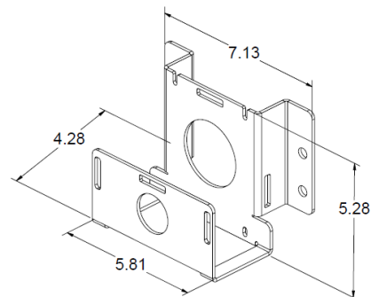
PTS5G-BK5165 Triplexer Bracket 1.0 lbs
