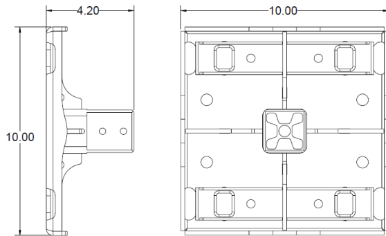
PTS5G-BK5130 Flat Bracket 3.7 lbs
