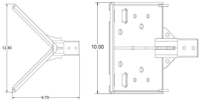
PTS5G-BK5131 Corner Bracket 4.8 lbs
