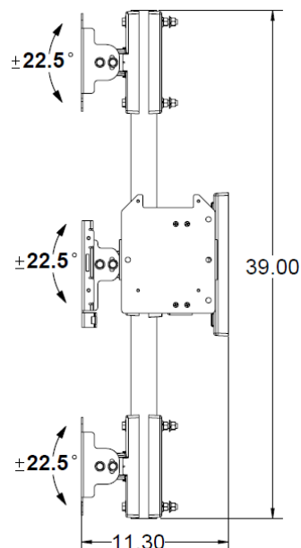
PTS5G-BK5203V-V2E Vertical Mount Views 16.8 lbs
