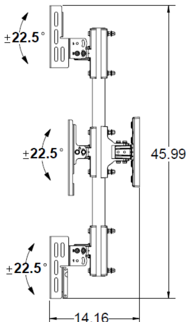
PTS5G-BK5103-V2N Vertical Mount Views
