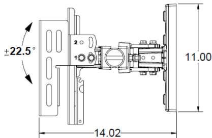
PTS5G-BK5103-V2N Vertical Mount Views
