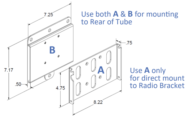
PTS5G-BK5144, 1.1lbs A & B included in 5103-V2N, A included in 5101-V2N
