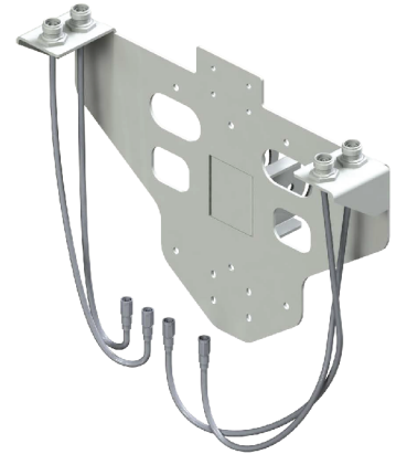
PTS5G-BK5111 (SAP 33871) OMNI Bracket, Supports 2 Dual 2 GHz Omni Antennas
