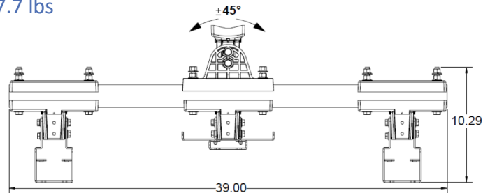
PTS5G-BK5103-V2N Horizontal Mount Views
