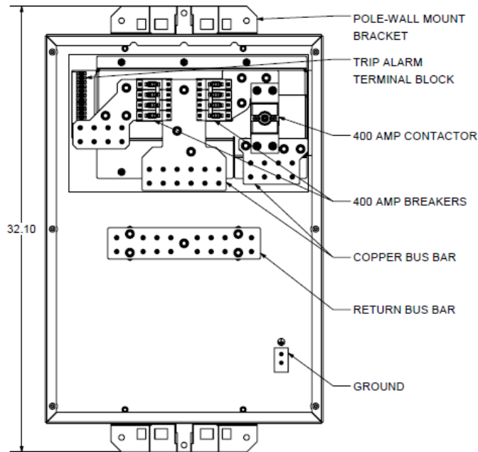
PTS31468-44A-C Internal view (shown with Contactor on right leg)
