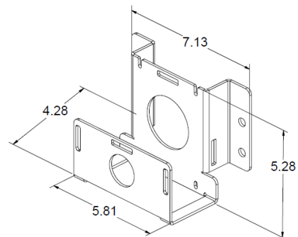
PTS5G-BK5165 Triplexer Bracket 1.0 lbs
