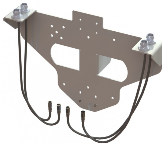
PTS5G-BK5111 (NOKIA OMNI) SAP.33871 PTS5G-BK5112 (ERICSSON OMNI) SAP.33872 PTS5G-BK5114 (Nokia LAA Omni) SAP TBD PTS5G-BK5115 (ERICSSON LAA Omni) SAP TBD
