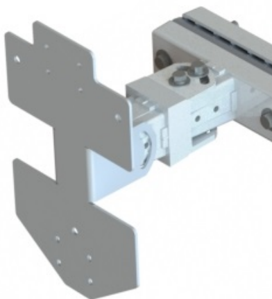
PTS5G-BK5110 UNIVERSAL BRACKET, TEE & PIVOT SAP.33870
