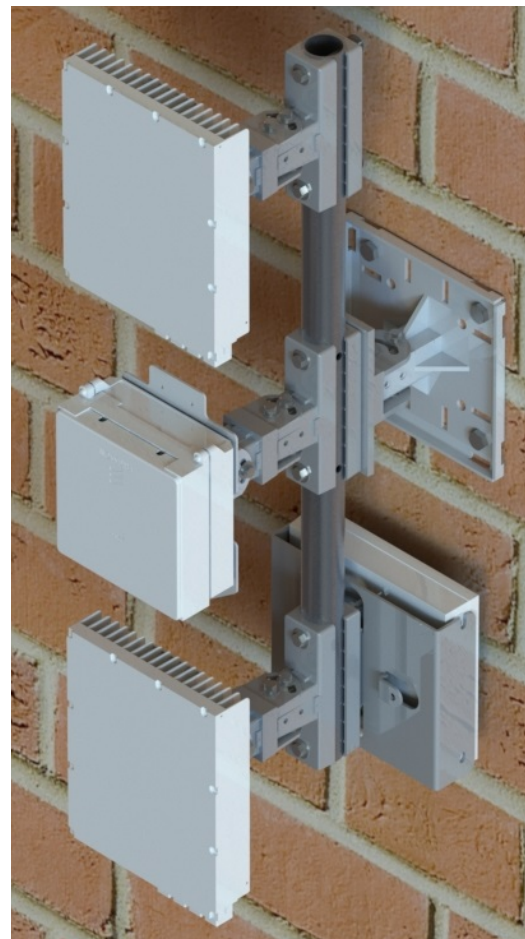
PTS5G-BK5103 MOUNTED VERTICAL utilizing MIXED RADIOS shown with included SAR-O Bracket and optional PTS5G-BK5130 WALL Mount
